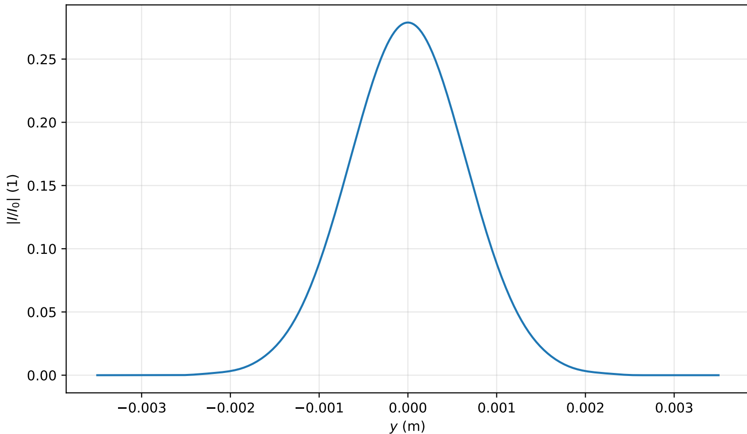
Intensity profile I(x=0, y, z=3.423)/I_0 , P_{in}=0.1P_{cr} , artificial time
